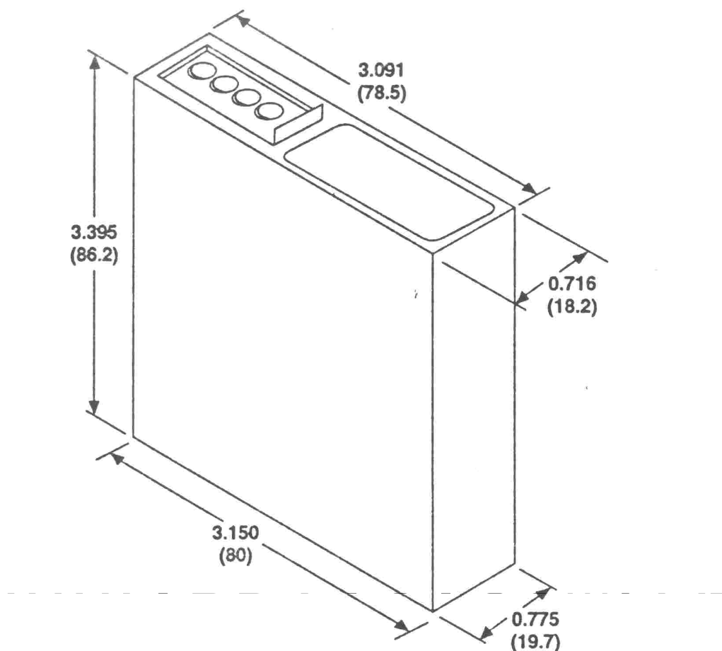
Figure 5. Outline Dimensions
