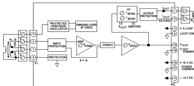
Figure 1. 3B17 Functional Block Diagram
