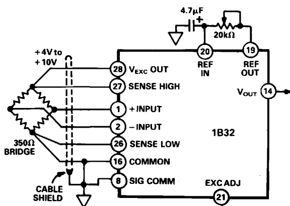
Figure 5. Constant Voltage Excitation: +4V to +10V Range.
