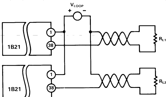
Figure 5. Multiple 1B21s with Single Loop Supply
