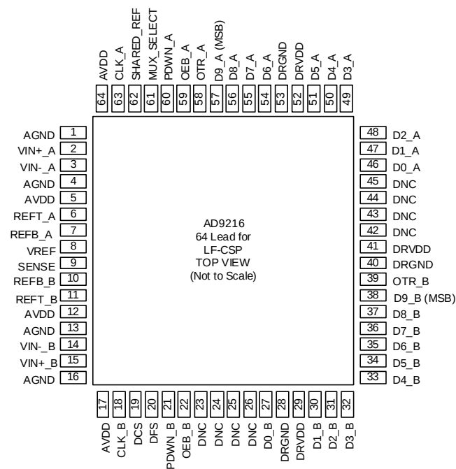
Figure 3. Pin Configuration
