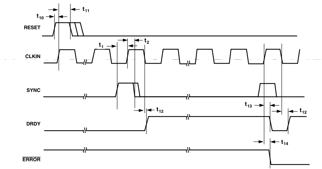
Figure 4. AD1556 RESET, DRDY, and Overwrite Timings
