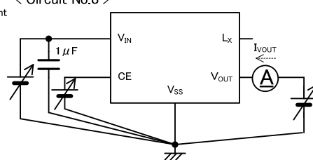
< Circuit No.8 >
