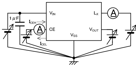
< Circuit No.5 >
