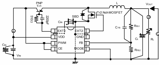
Circuit ③
