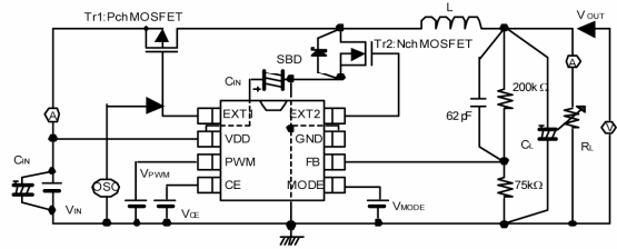
Circuit ④
