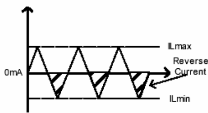
Coil current when synchronous
