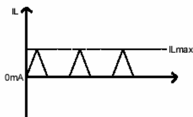
Coil current when non-synchronous (DiscontinuousMode)
