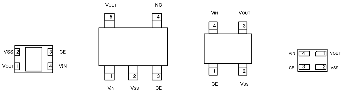
USP-4 (BOTTOM VIEW)
