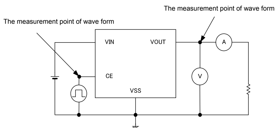
Circuit ⑤
