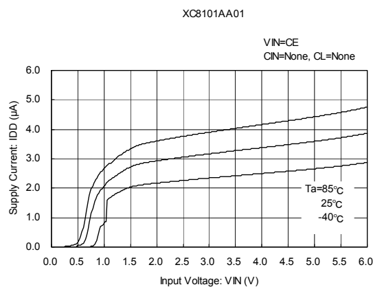
(3) Supply Current vs. Input Voltage
