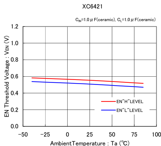
(7) EN Threshold Voltage vs. Ambient Temperature
