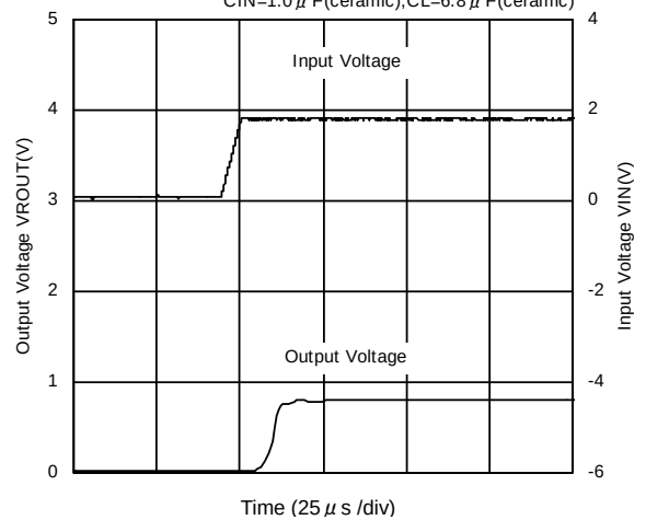
XC6402 Series (VR: 3.0V)
