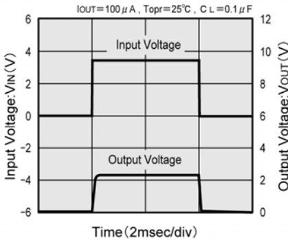
XC62RP2502 (2.5 V)
