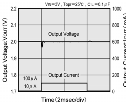
XC62RP2002 (2 V)
