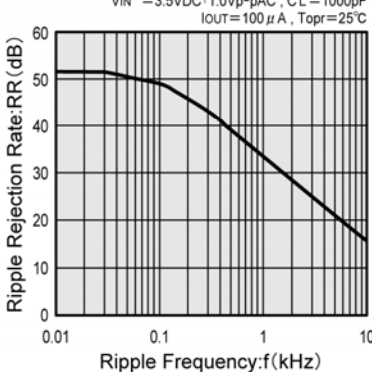
XC62RP2502 (2.5 V)
