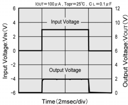
XC62RP2002 (2 V)
