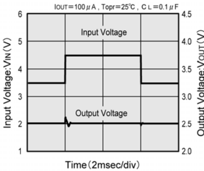
XC62RP2502 (2.5 V)
