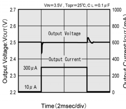
XC62RP2502 (2.5 V)
