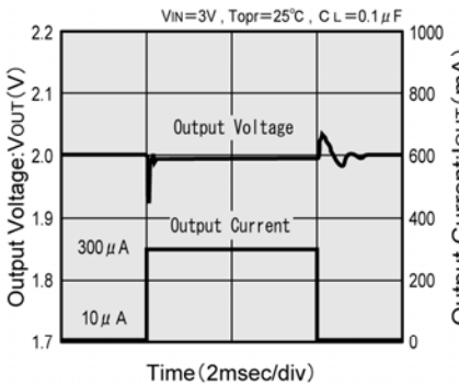
XC62RP2002 (2 V)
