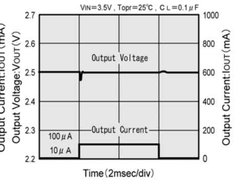
XC62RP2502 (2.5 V)
