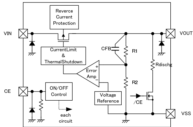
XC6222Dseries
