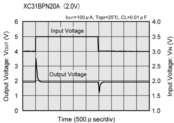
(5) Input Transient Response 2
