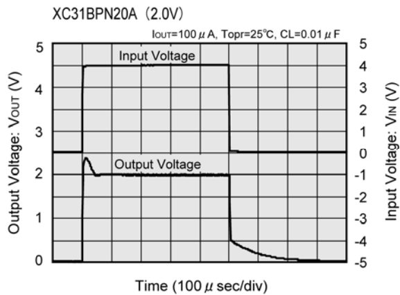
(4) Input Transient Response 1
