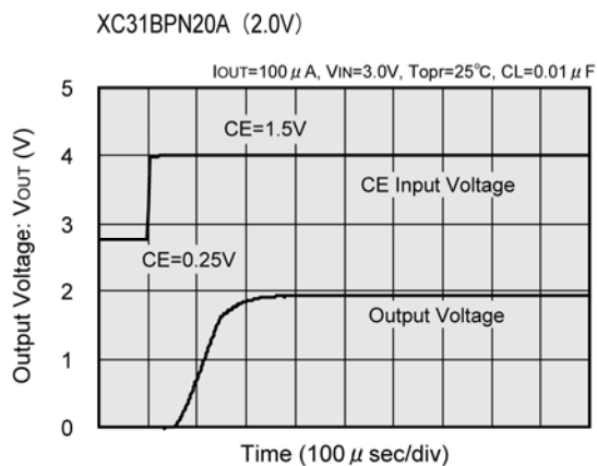
(6) CE Pin Transient Response
