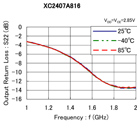
(22) Output Return Loss vs. Frequency
