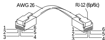
Telejack connectors
