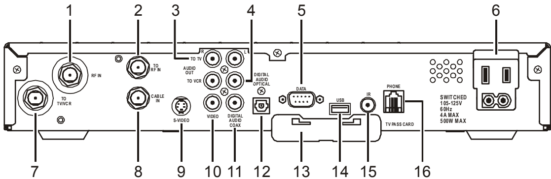
Figure 2-2 Rear panel
