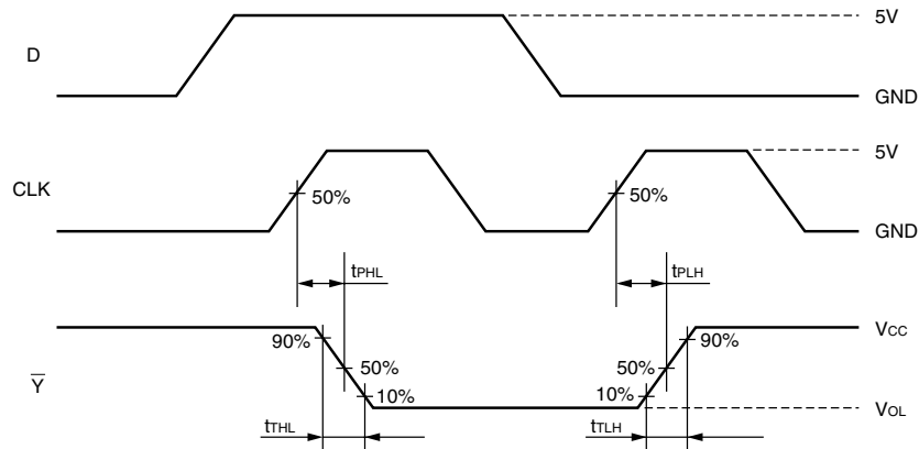
SWITCHING TIMES
