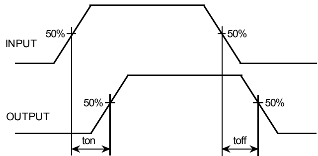
TIMING DIAGRAM
