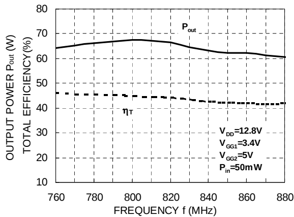
OUTPUT POWER, TOTAL EFFICIENCY, versus FREQUENCY
