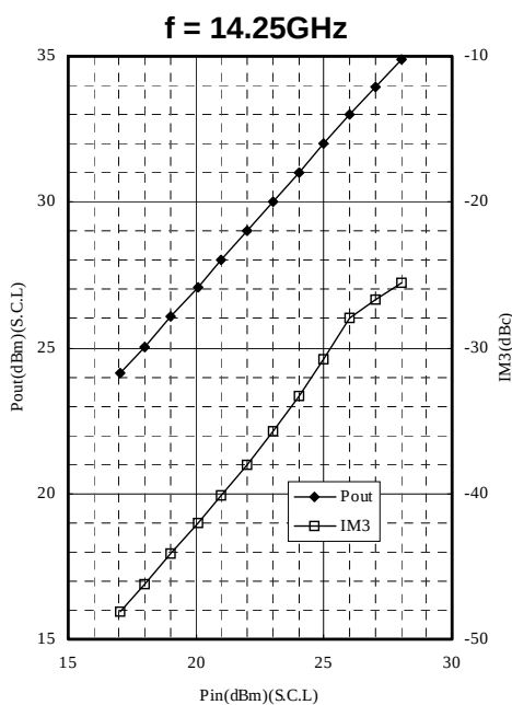
Pout, IM3 vs. Pin
