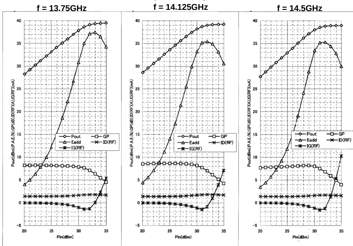
Pout, Glp, PAE, Id, Ig vs. Pin
