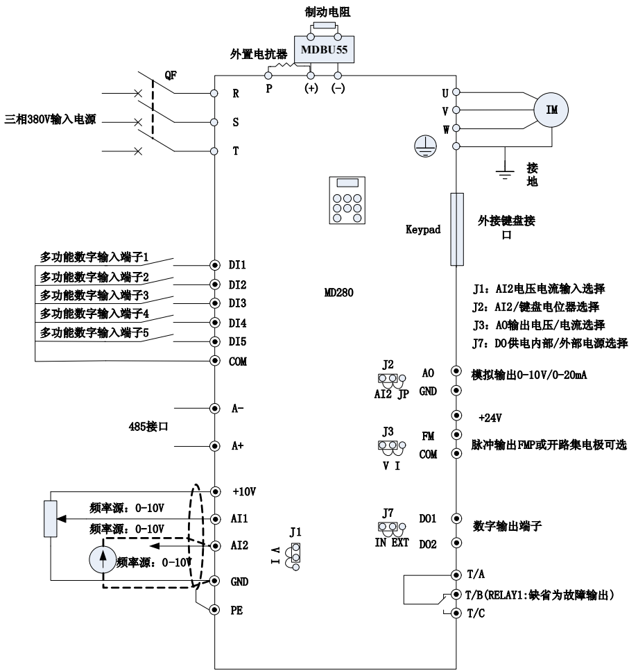
图3-7 MD280T75G/90P~MD280T400G/450P外置电抗器接线示意图
