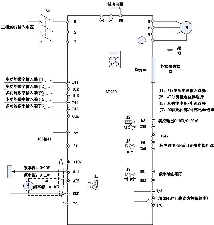
图3-5 MD280T0.7G~MD280T30G/37P三相变频器接线示意图
