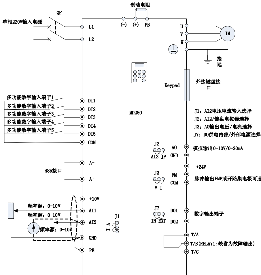
图3-4 MD280S0.4G/MD280S0.7G/MD280S1.5G/MD280S2.2G
