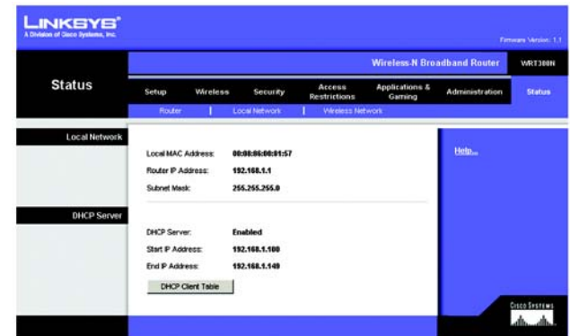
Figure 5-51: Status Tab - Local Network
