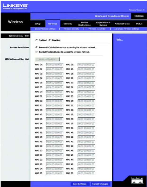
Figure 5-23: Wireless Tab - Wireless MAC Filter
