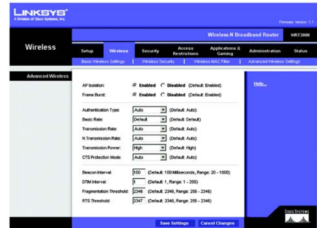
Figure 5-25: Wireless Tab - Advanced Wireless Settings
