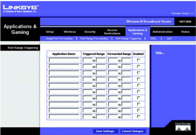
Figure 5-33: Applications & Gaming Tab - Port Range Triggering
