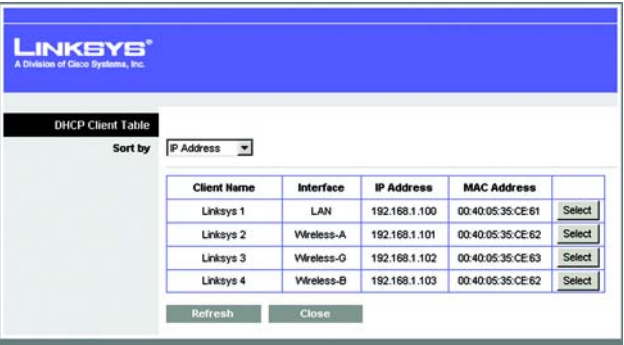
Figure 5-35: DHCP Client Table
