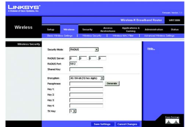
Figure 5-21: Wireless Security - RADIUS
