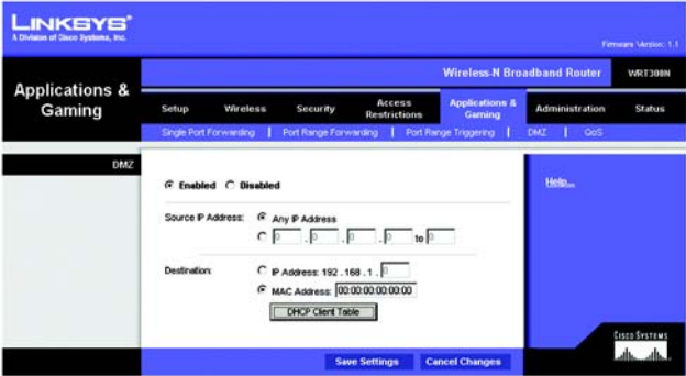
Figure 5-34: Applications & Gaming Tab - DMZ
