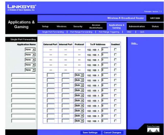
Figure 5-31: Applications & Gaming Tab - Single Port Forwarding
