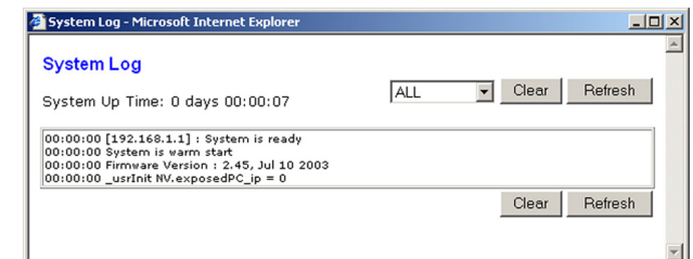
Figure 5-27: System Log
