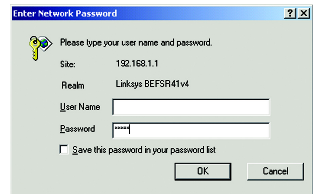
Figure 5-2: Router Login
