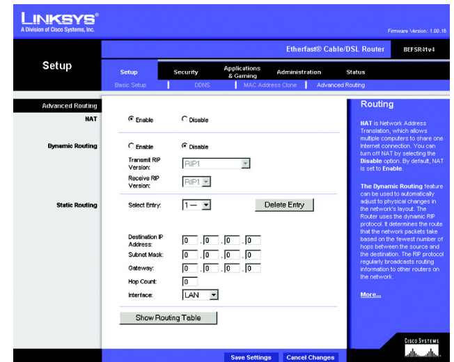
Figure 5-13: Setup Tab - Advanced Routing
