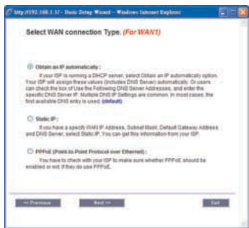
WAN Connection Type
