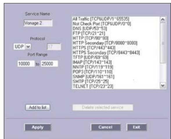
Add Vonage 2 Service
