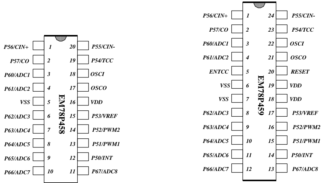
Fig. 1 Pin Assignment
