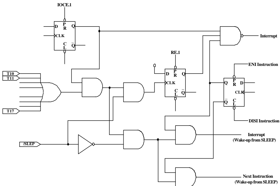
Fig. 9 Block Diagram of Port 6 with Input Changed Interrupt/Wake-up
