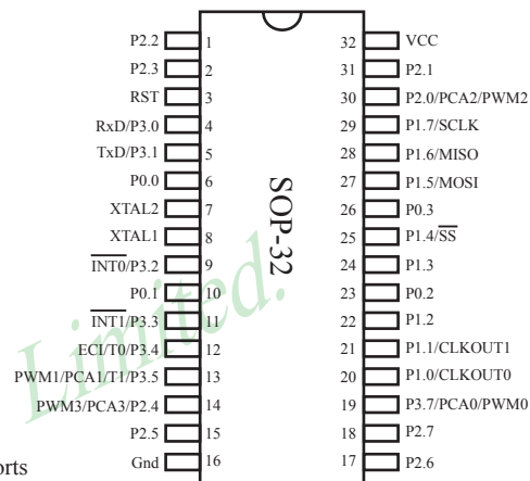
STC12C5410 series (without A/D Converter), SOP-32
