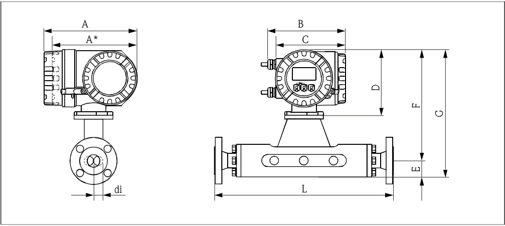
Promass M
