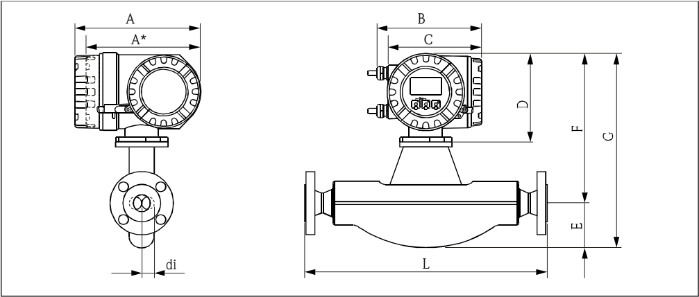
Promass F
