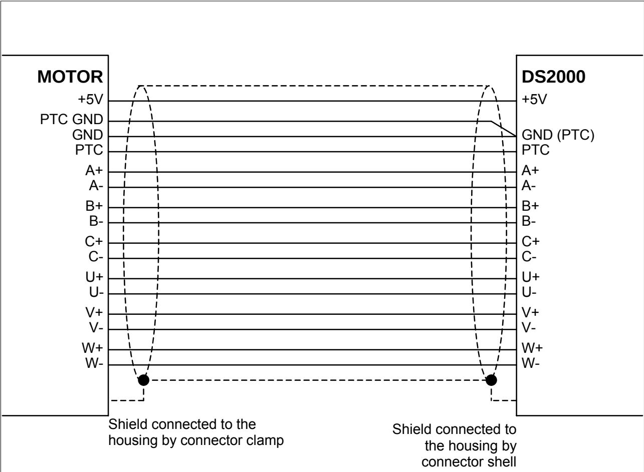
Fig. 2.13 – Encoder connections
