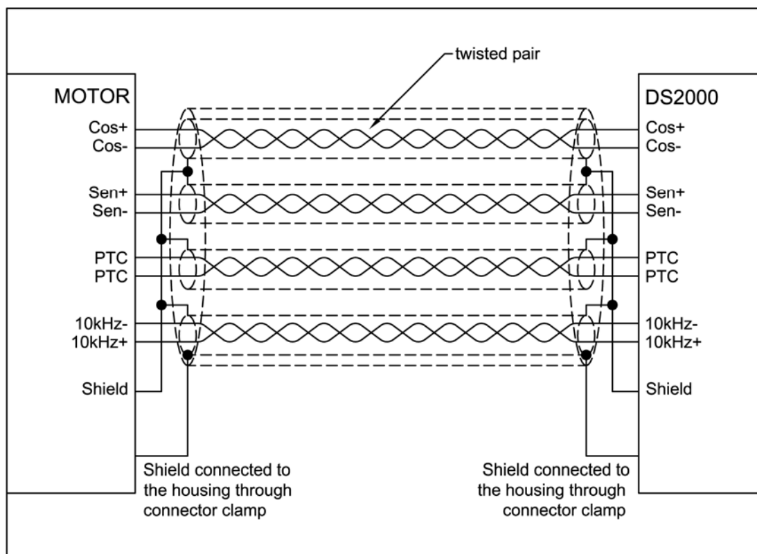
Fig. 2.14 – Resolver connections
