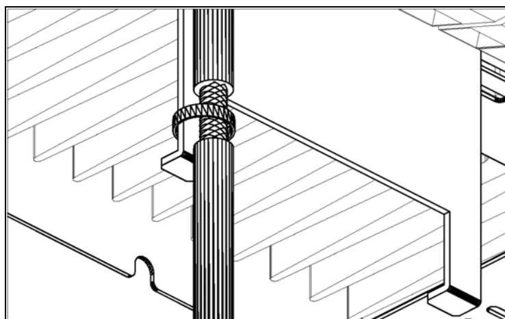
Fig. 3.2 – Grounding of shield without metallic connector
