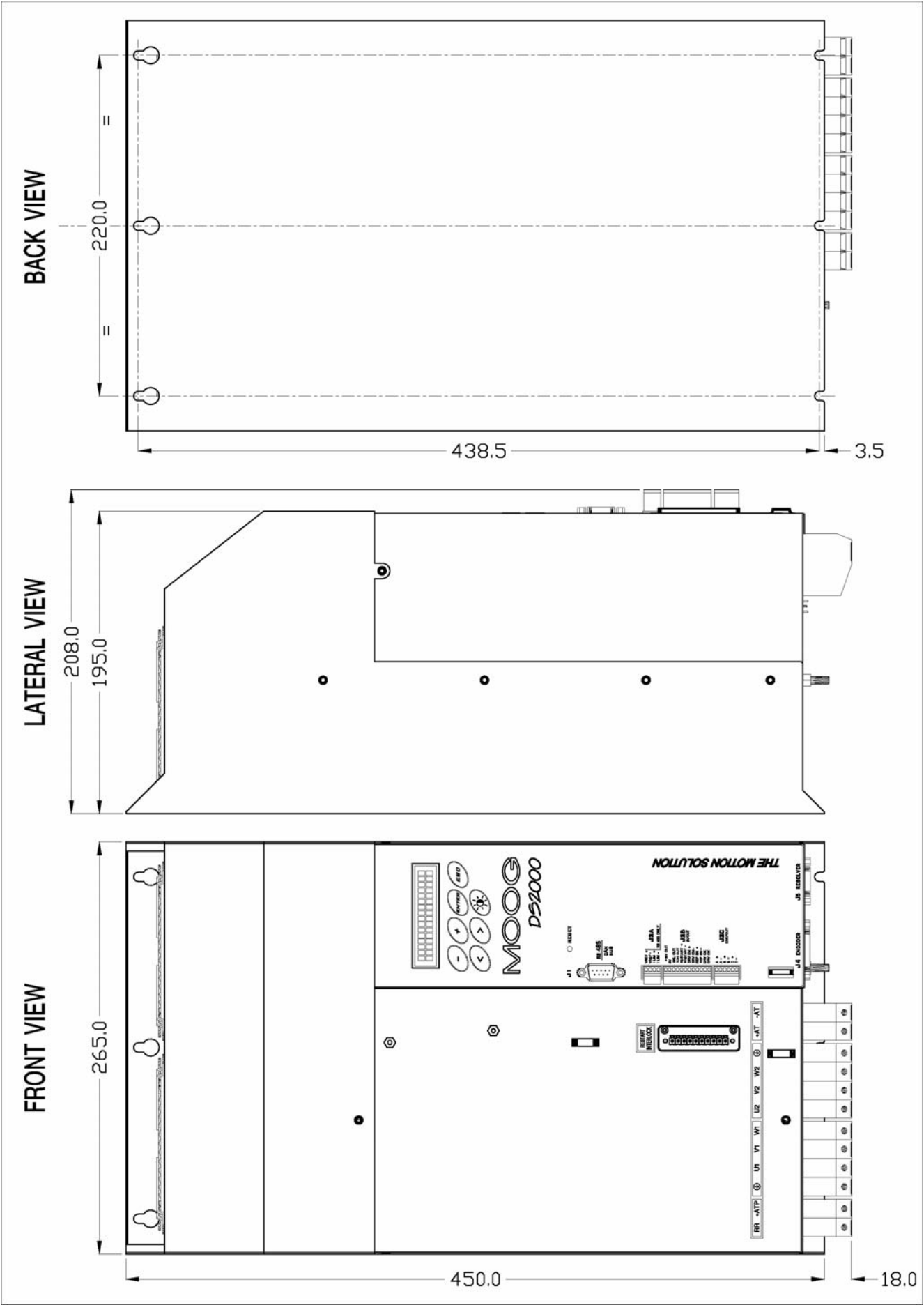
Fig. 2.4 – Size D dimensions and drilling jig (mm)
