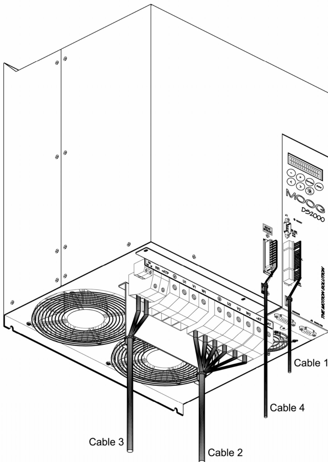
Fig. 3.5.1 – E size connections drive side
