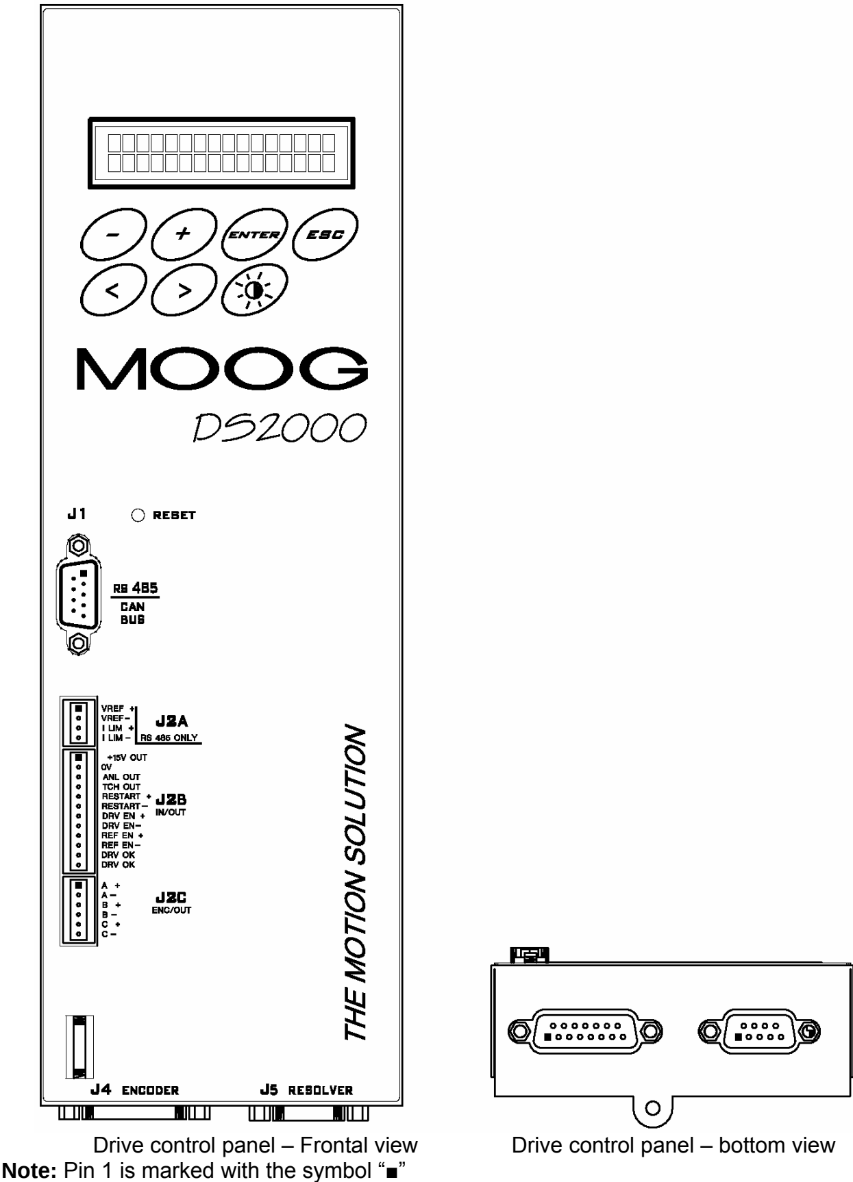
Fig. 2.10 – Control card connectors
