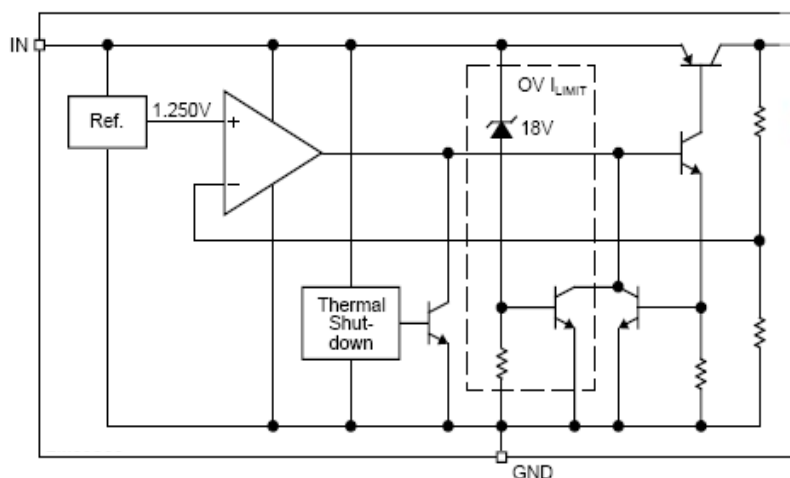
LM39500 Fixed (1.5V, 1.8V, 2.5V, 3.3V, 5.0V)
