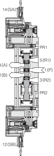
G113-4E2-14
