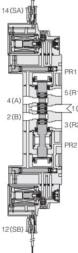
G113-4E2
