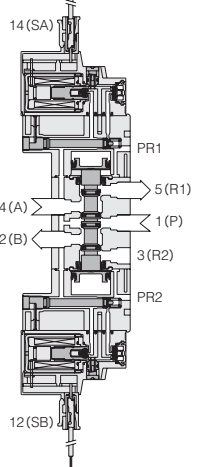
G110-4E2
