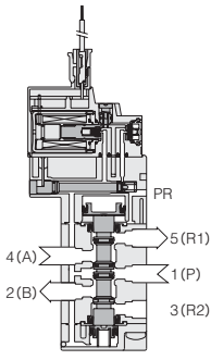
G110-4E1
