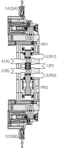
G113-4E2-13
