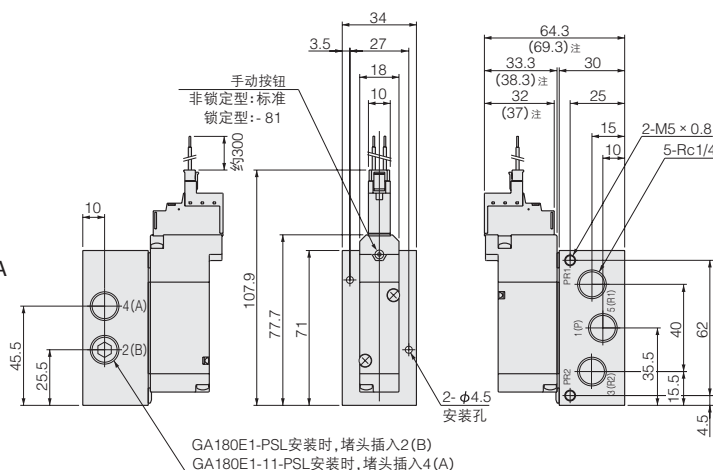
GA180E1-25-PSL GA180-4E1-25-PSL
