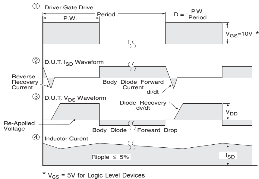
Fig 15. For N-Channel Power MOSFETs
