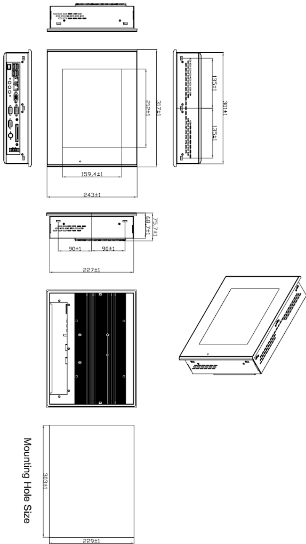
Figure 1.3: Dimensions of the EX-96107A+
