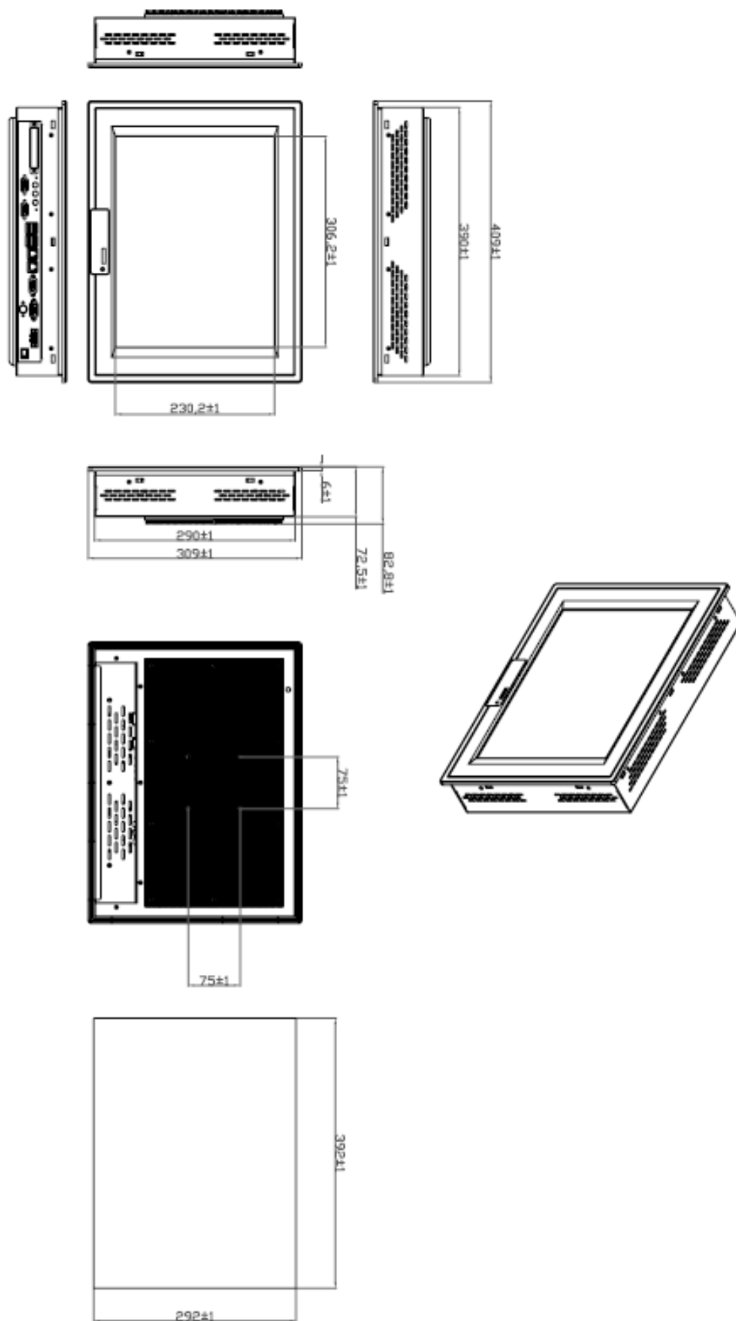
Figure 1.5: Dimensions of the EX-96157A+
