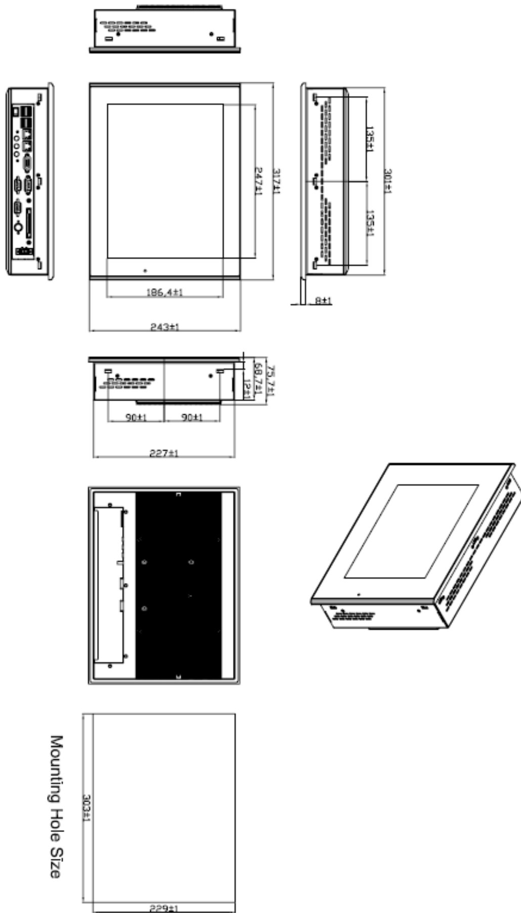
Figure 1.4: Dimensions of the EX-96127A+
