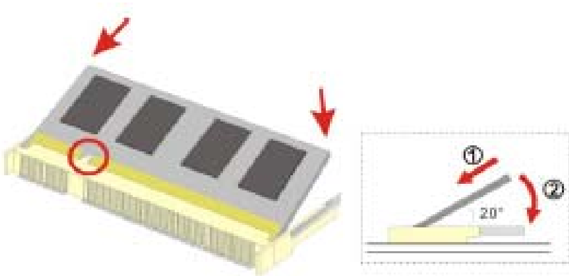
Figure 2.2: Installation of Memory Module
