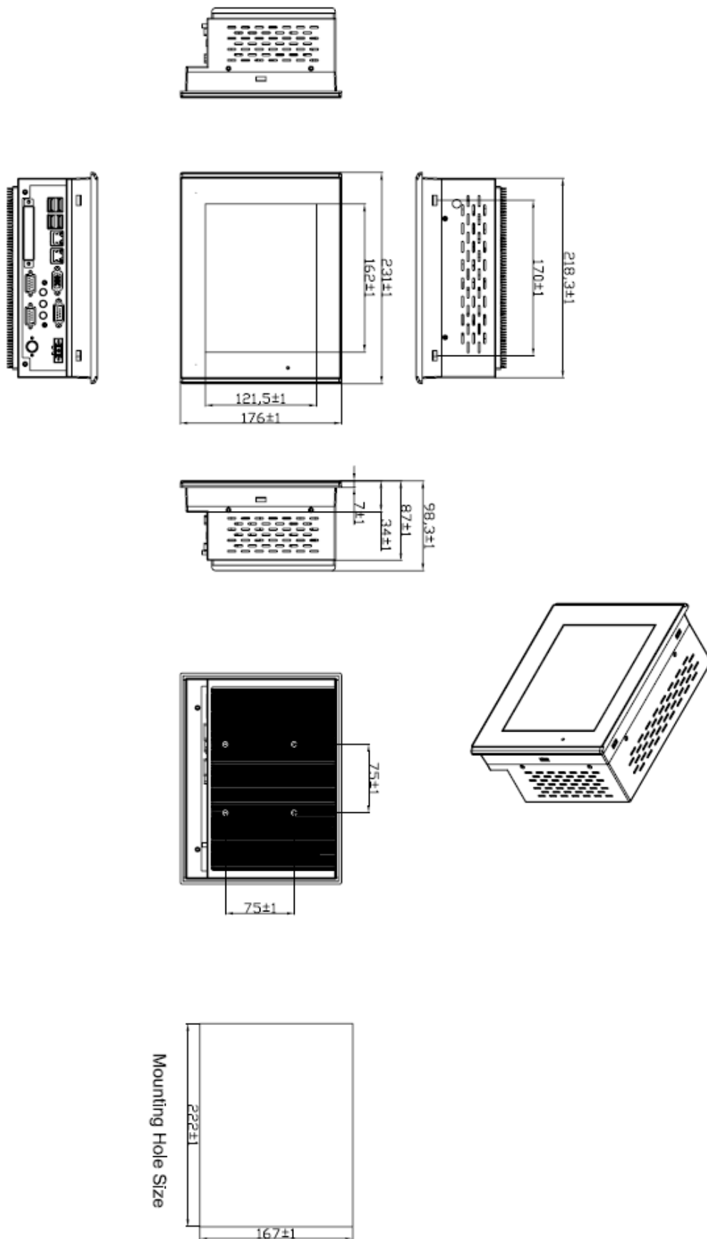
Figure 1.2: Dimensions of the EX-96087A+
