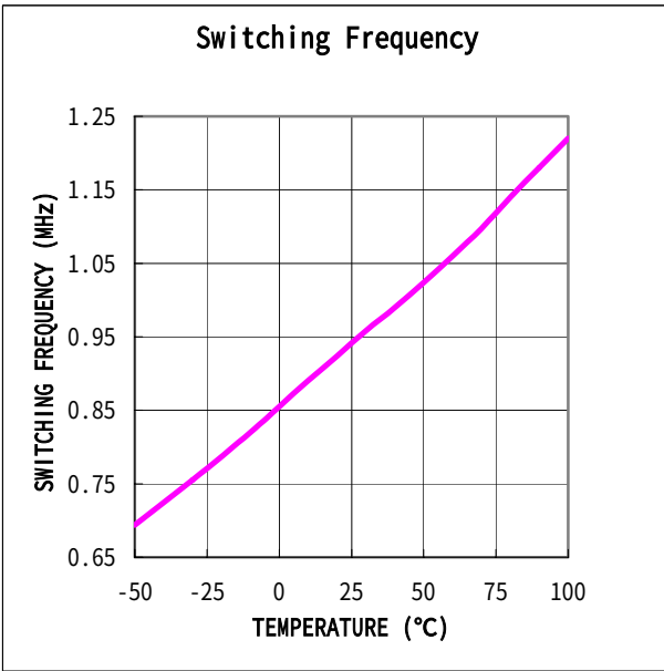
(5) Frequency vs Temperature (Vin=3.6V)
