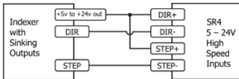
Connecting to Indexer with Sinking Outputs
