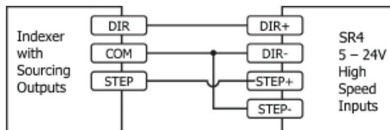
Connecting to Indexer with Sourcing Outputs
