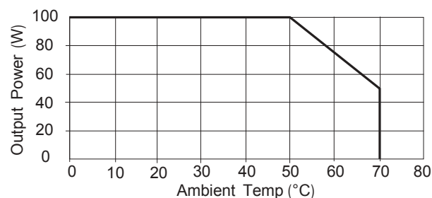
Fan-cooled with 10 CFM
