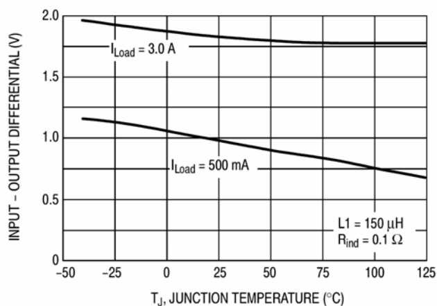
Figure 4. Dropout Voltage
