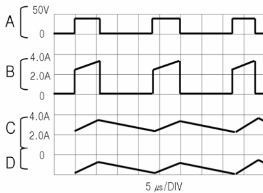
Figure 13. Switching Waveforms
