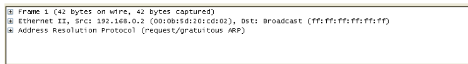
Figure 3.17. The "Packet Details" pane
