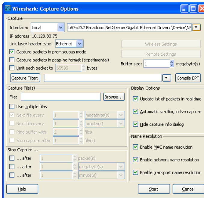
Figure 4.3. The "Capture Options" dialog box
