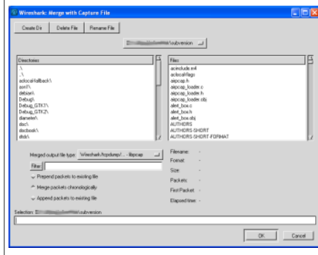
Figure 5.9. "Merge" - old GTK version
