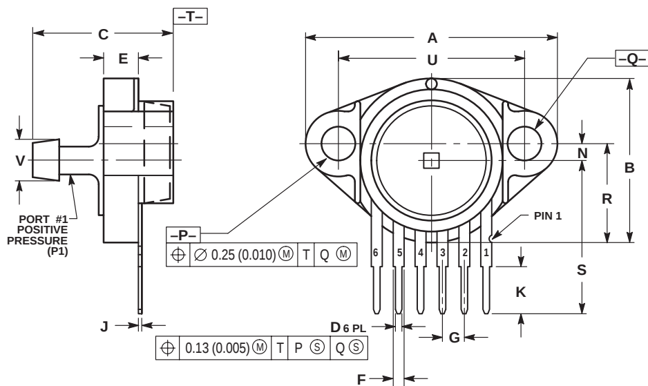
CASE 867F-03 ISSUE D
