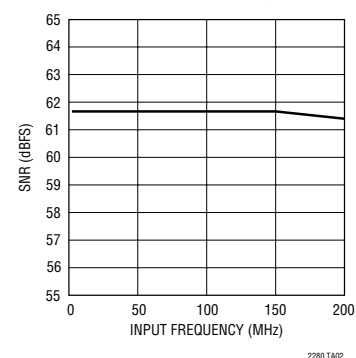
SNR vs Input Frequency, -1dB, 2V Range
