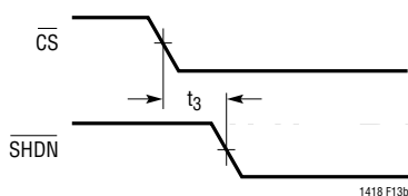
Figure 13b. \overline{CS} to \overline{SHDN} Timing
