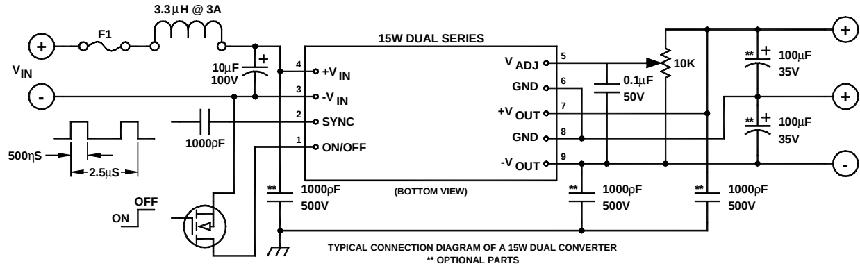
FIGURE 3. Dual converter
