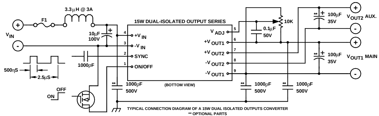
FIGURE 4. Dual isolated output converter
