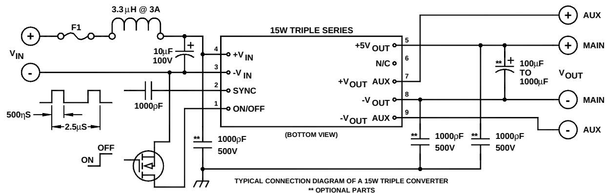
FIGURE 5. Triple converter
