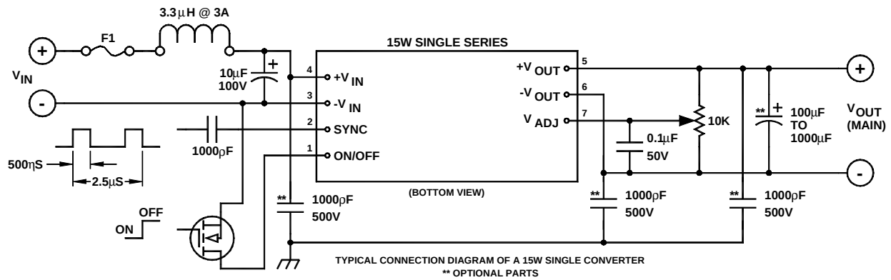
FIGURE 2. Single converter
