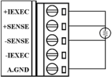
4-wire RTD 连接
