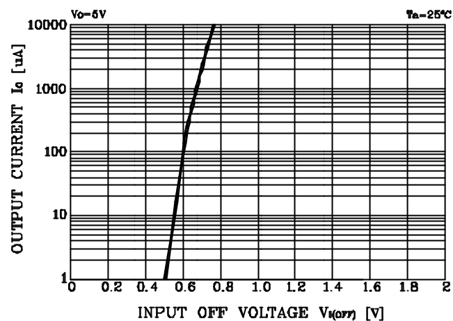
Fig. 2 I_O - V_{I(OFF)}
