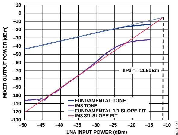
图31. LNA/混频器IIP3: V_{DD} = 3.0\text{ V} , 温度 = 25^{\circ}\text{C} , RF频率 = 915 MHz, LNA增益 = 低, 混频器增益 = 低, 信号源1频率 = (915 + 0.4)\text{ MHz} , 信号源2频率 = (915 + 0.7)\text{ MHz}
