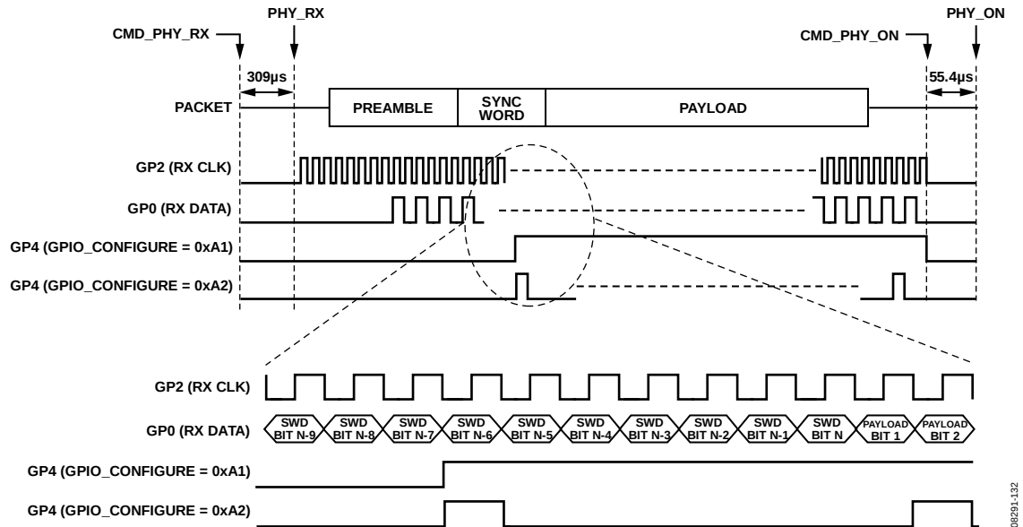
图84. Sport模式接收, DATA\_MODE = 2 且 GPIO\_CONFIGURE = 0xA1, 0xA2, 0xA4, 0xA5, 0xA7, 0xA8
