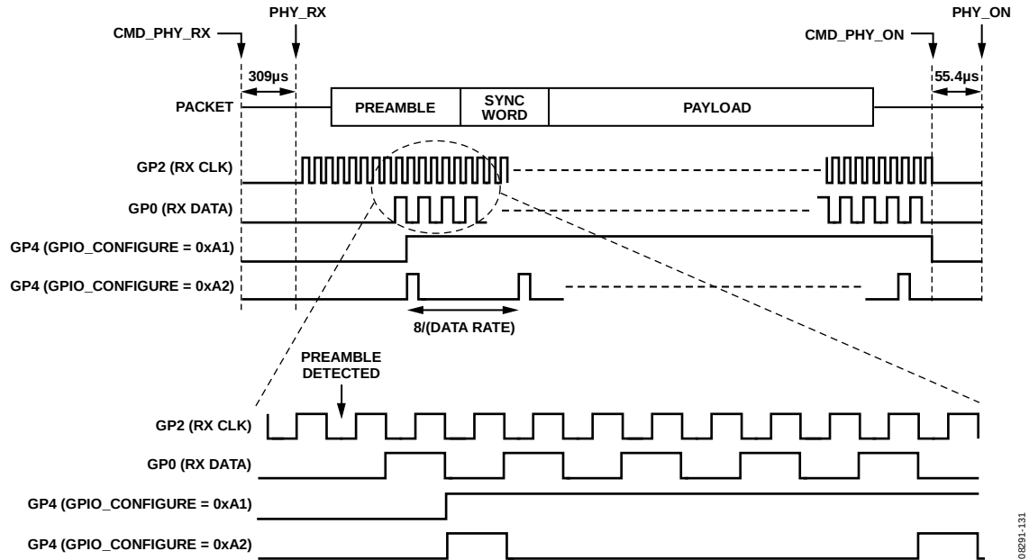
图83. Sport模式接收, DATA\_MODE = 1 且 GPIO\_CONFIGURE = 0xA1, 0xA2, 0xA4, 0xA5, 0xA7, 0xA8
