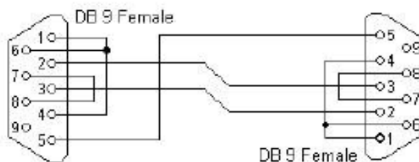
Null modem with loop back handshaking
