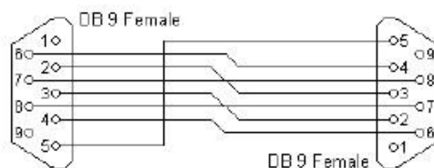
Null modem with full handshaking
