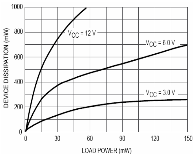
Figure 8. Device Dissipation, 8.0 \Omega Load
