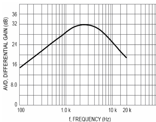
Figure 25. Frequency Response of Figure 24
