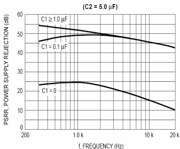
Figure 5. Power Supply Rejection versus Frequency
