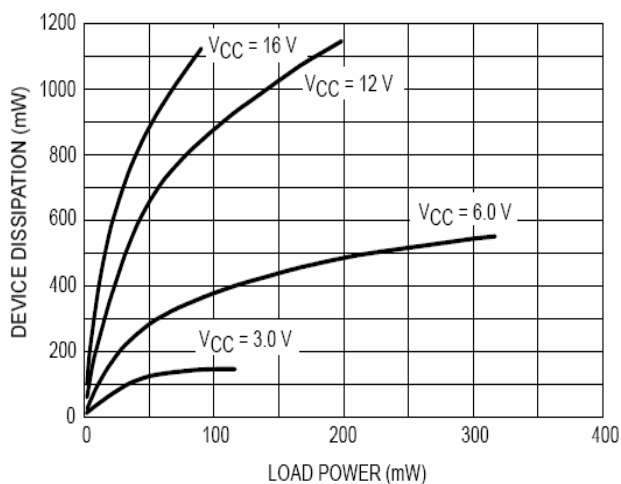
Figure 9. Device Dissipation, 16 \Omega Load
