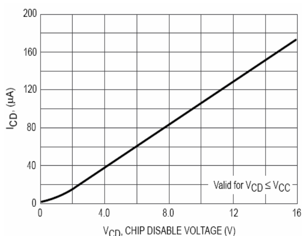
Figure 20. Input Characteristics @ CD (Pin 1)
