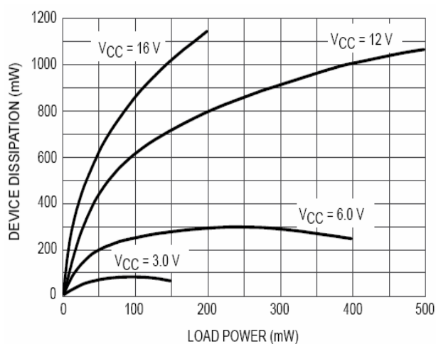
Figure 10. Device Dissipation, 32 \Omega Load
