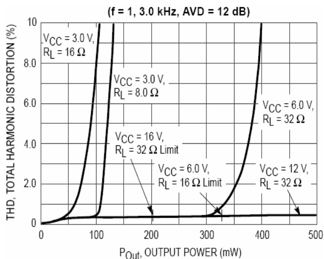
Figure 13. Distortion versus Power
