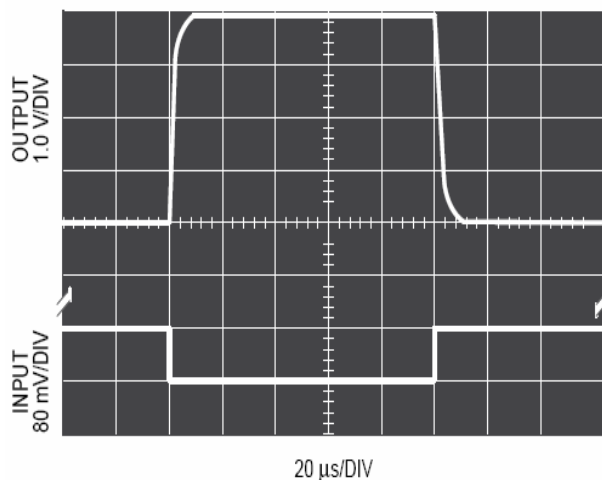
Figure 17. Large Signal Response
