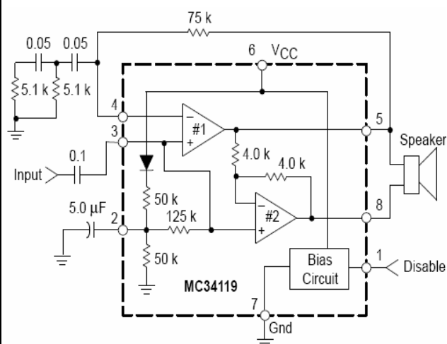
Figure 22. Audio Amplifier with Bass Suppression
