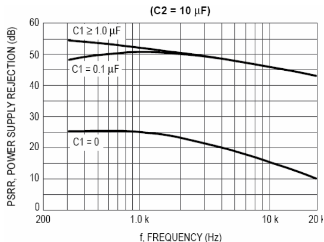
Figure 4. Power Supply Rejection versus Frequency
