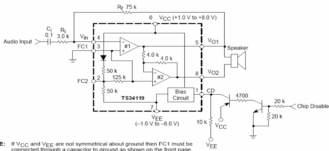
Figure 26. Split Supply Operation
