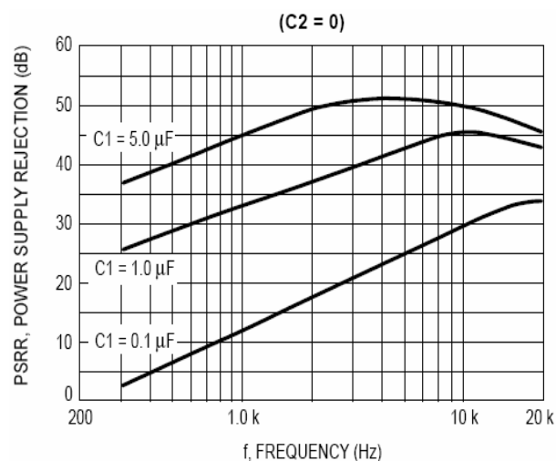
Figure 7. Power Supply Rejection versus Frequency
