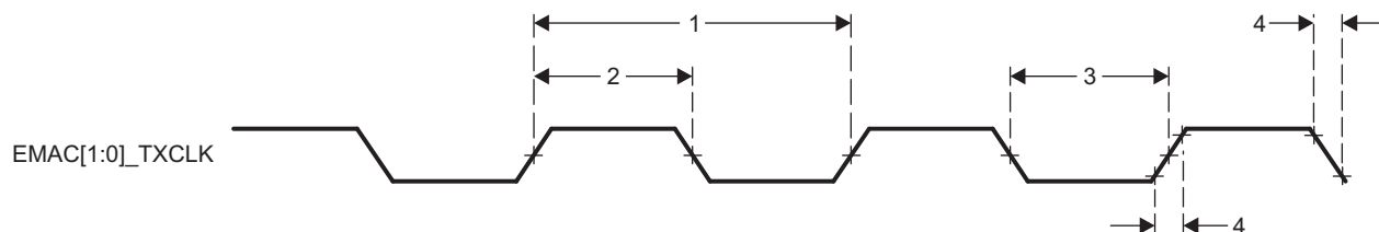
Figure 8-45. EMAC[1:0]_TXCLK Timing
