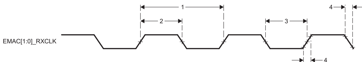
Figure 8-44. EMAC[1:0]_RXCLK Timing
