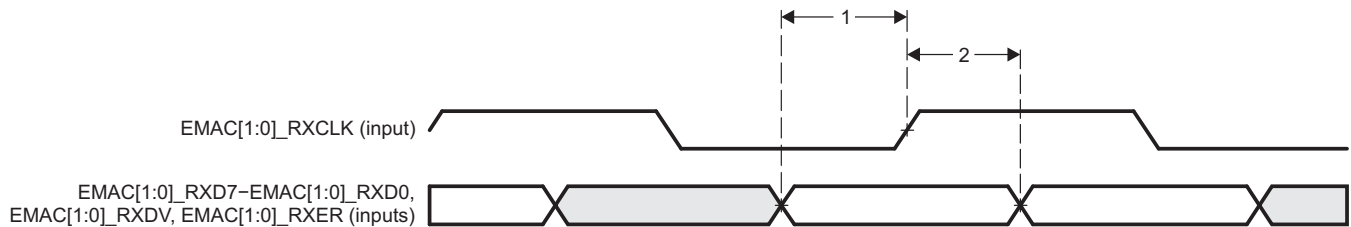
Figure 8-46. EMAC Receive Timing
