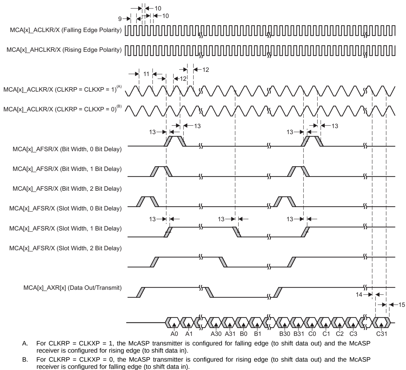
Figure 8-75. McASP Output Timing
