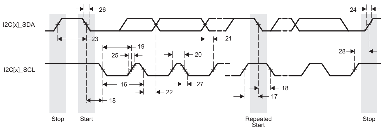
Figure 8-73. I2C Transmit Timing
