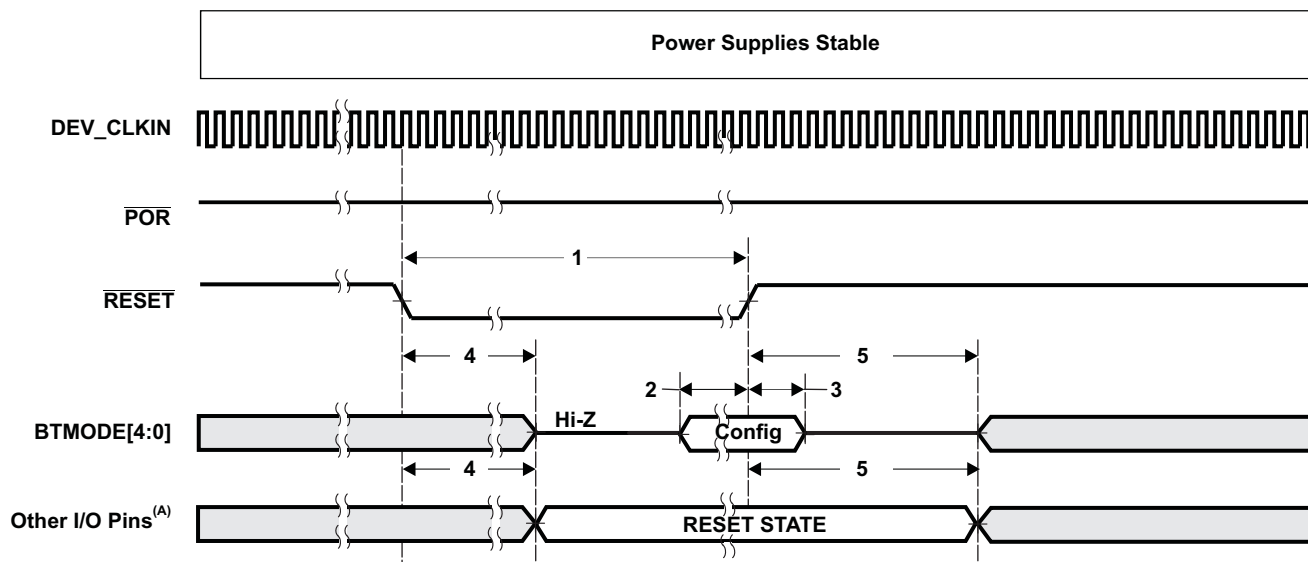
Figure 7-3. Warm Reset ( \overline{\text{RESET}} ) Timing
