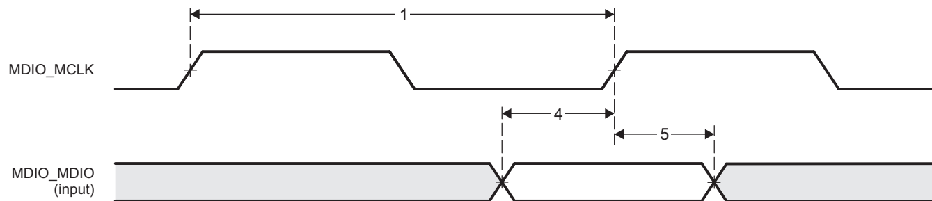
Figure 8-48. MDIO Input Timing
