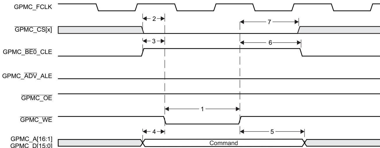
Figure 8-63. GPMC/NAND Flash - Command Latch Cycle Timing
