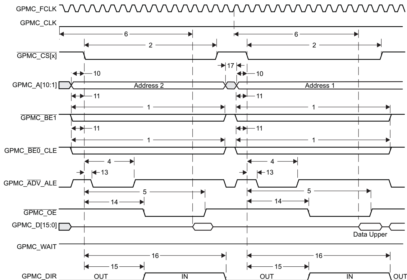
Figure 8-58. GPMC Non-Multiplexed NOR Flash - Asynchronous Read - 32-Bit Timing
