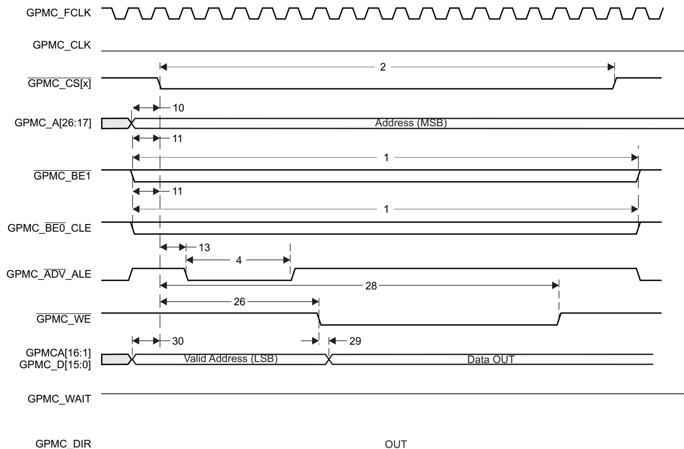
Figure 8-62. GPMC Multiplexed NOR Flash - Asynchronous Write - Single Word Timing
