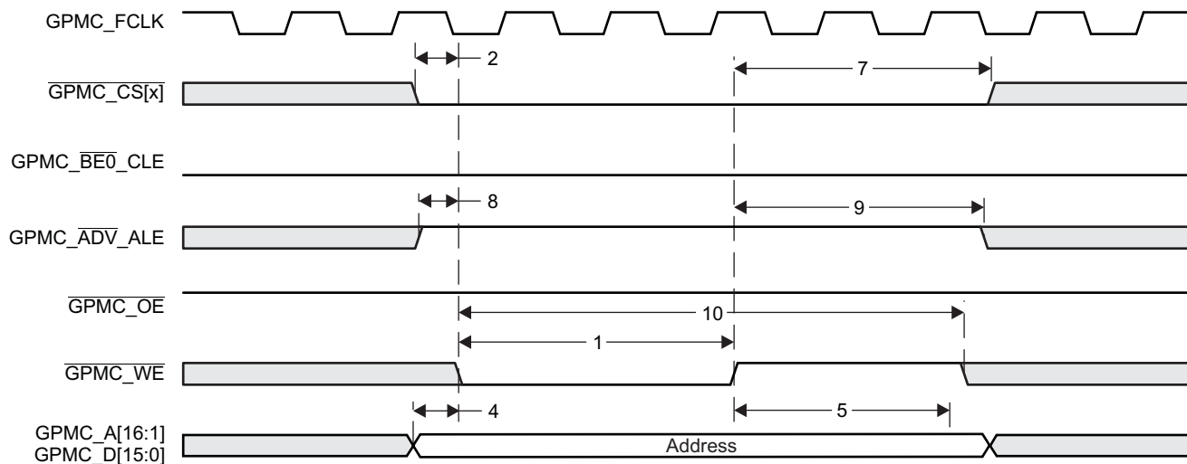
Figure 8-64. GPMC/NAND Flash - Address Latch Cycle Timing
