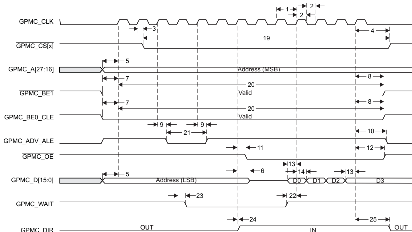
Figure 8-55. GPMC Multiplexed NOR Flash - 4x16-bit Synchronous Burst Read (GPMCFCLKDIVIDER = 0)
